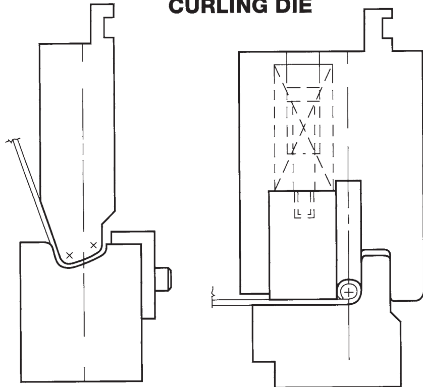
Example of a Special Die Modified for European Brake
